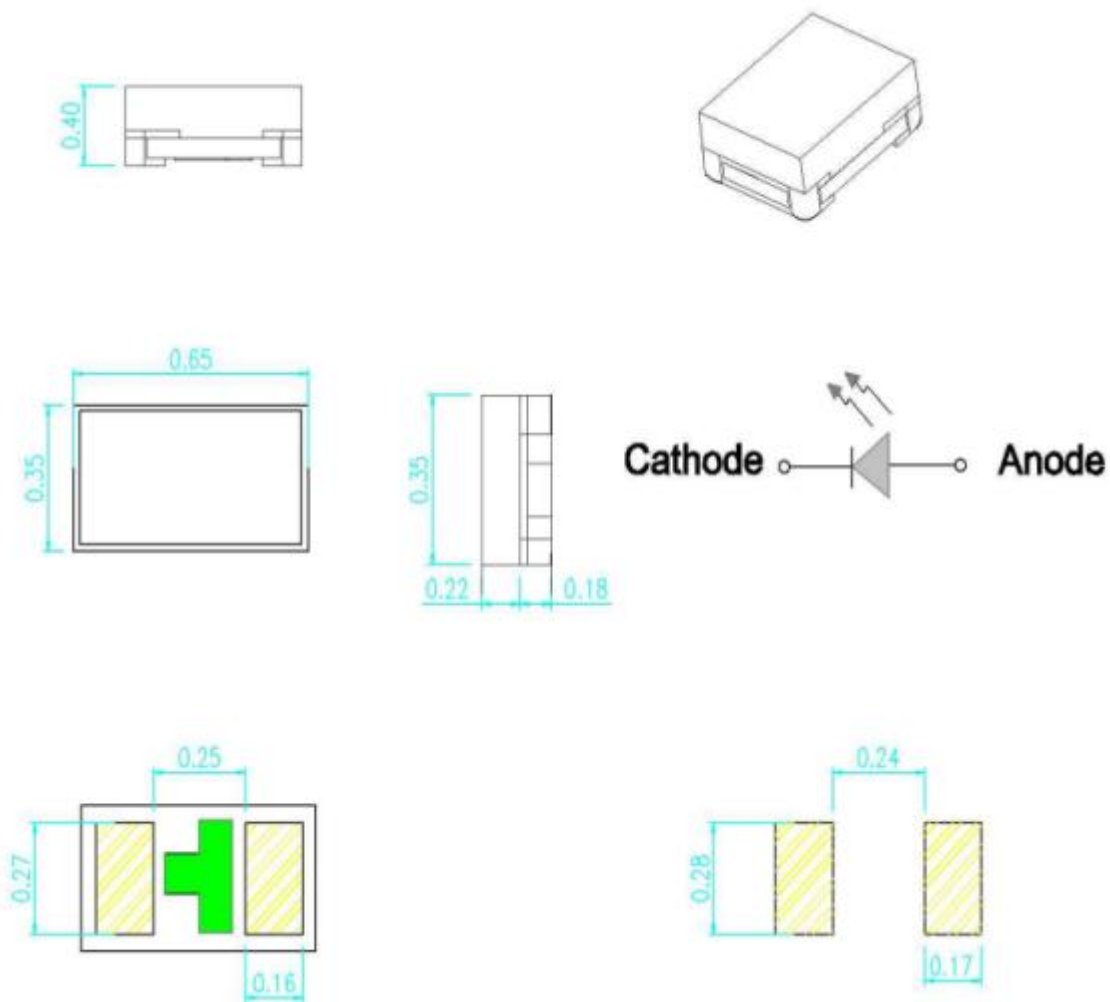
建议焊盘尺寸 Recommended pad size
