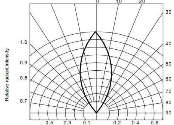
Fig.6 Radiation diagram
