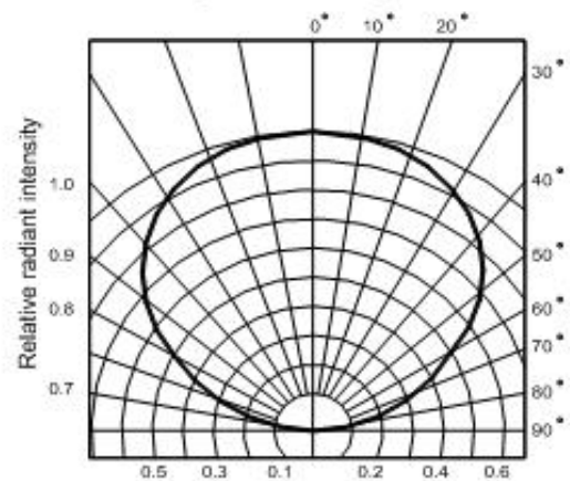
Fig.6 Radiation diagram
