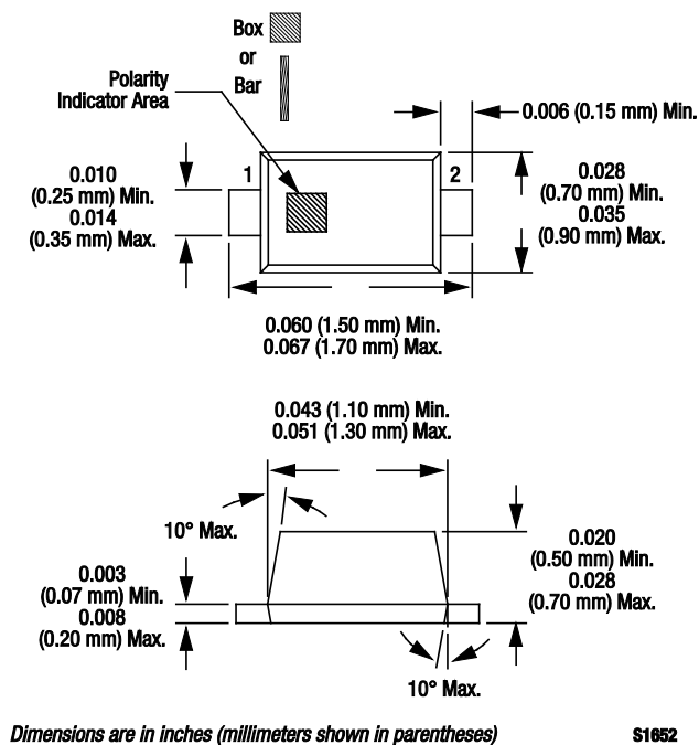
Figure 3. SC-79 Package Dimensions
