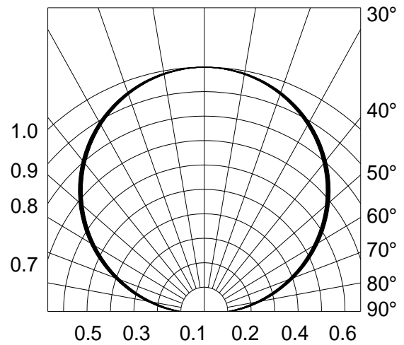
Fig.6-Radiation Diagram T_a=25^\circ\text{C}
