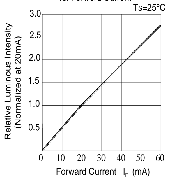
Fig.2-Relative Luminous Intensity vs. Forward Current Ts=25°C
