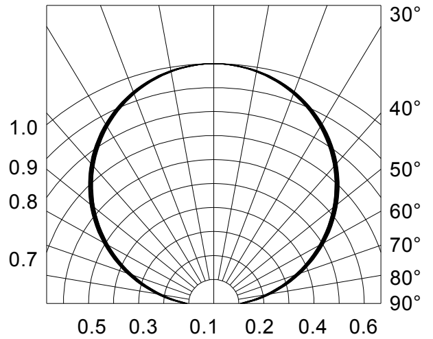
Fig.6-Radiation Diagram T a =25°C
