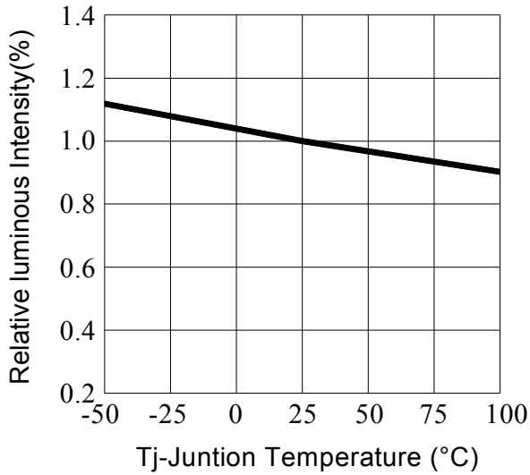
Fig.3-Relative Luminous Intensity vs.Juntion Temperature
