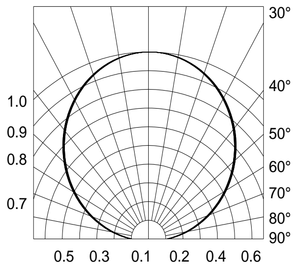
Fig.6-Radiation Diagram Ta=25°C
