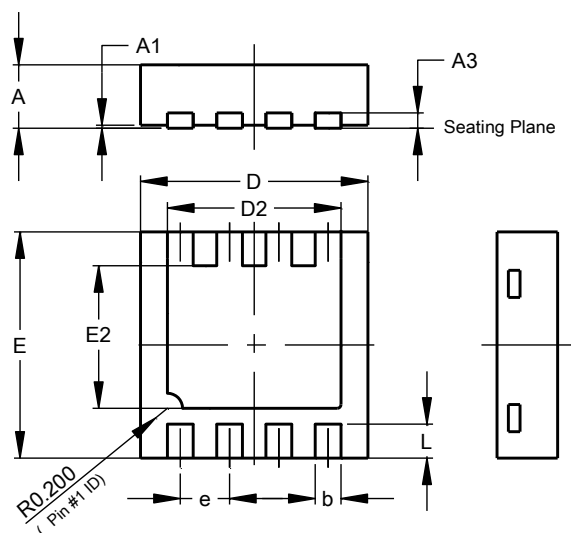
U-DFN3030-8
