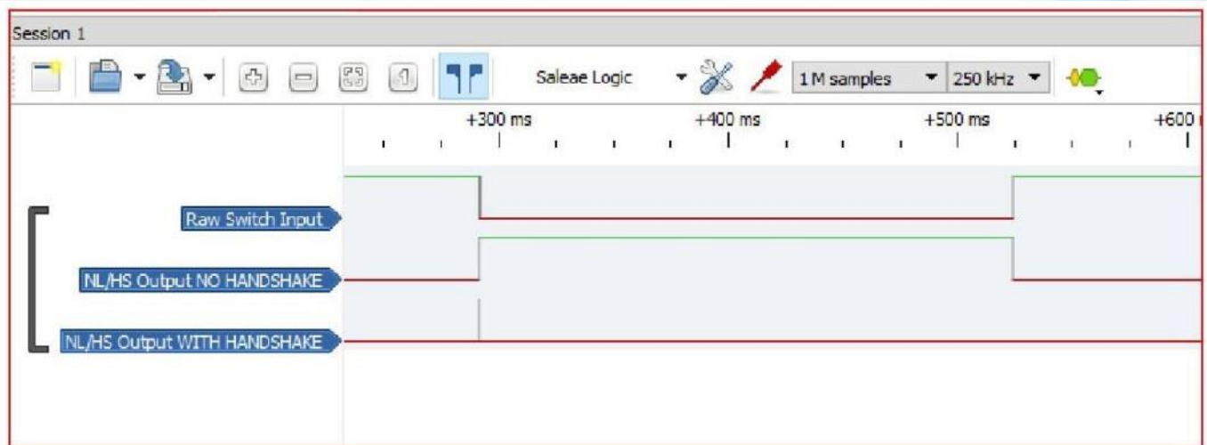
Figure 1. LS100 Series Logic Analyzer Capture of Switch Cycle With/Without Handshake
