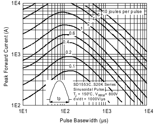
Fig. 28 - Maximum Total Energy Loss Per Pulse Characteristics
