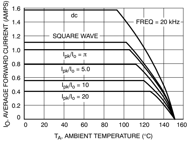
Figure 19. Current Derating
