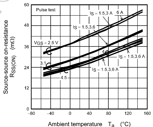
Fig. 10.6 R_{SS(ON)} - T_a (Note 6)
