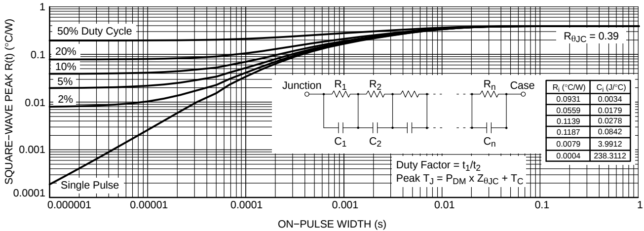
Figure 9. IGBT Die Self-heating Square-wave Duty Cycle Transient Thermal Response
