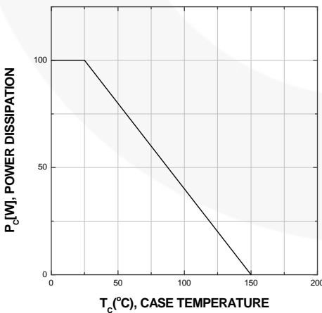
Figure 17. Power Derating
