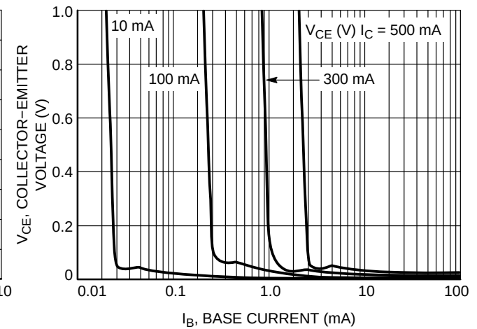
Figure 6. Saturation Region
