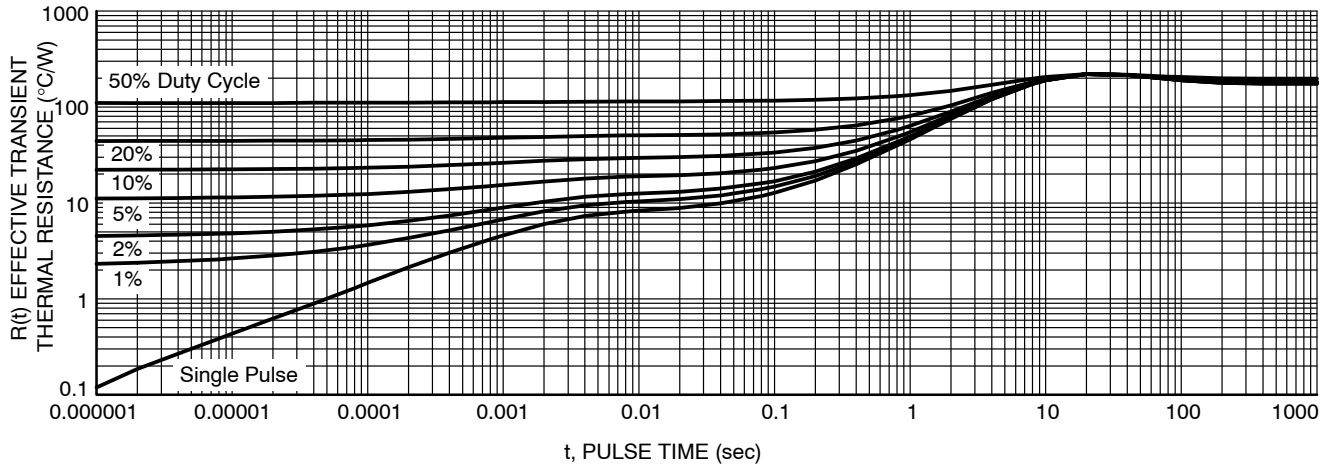
Figure 2. Thermal Resistance (FR-4 @ 7.6 mm², 1 oz. Cu trace)
