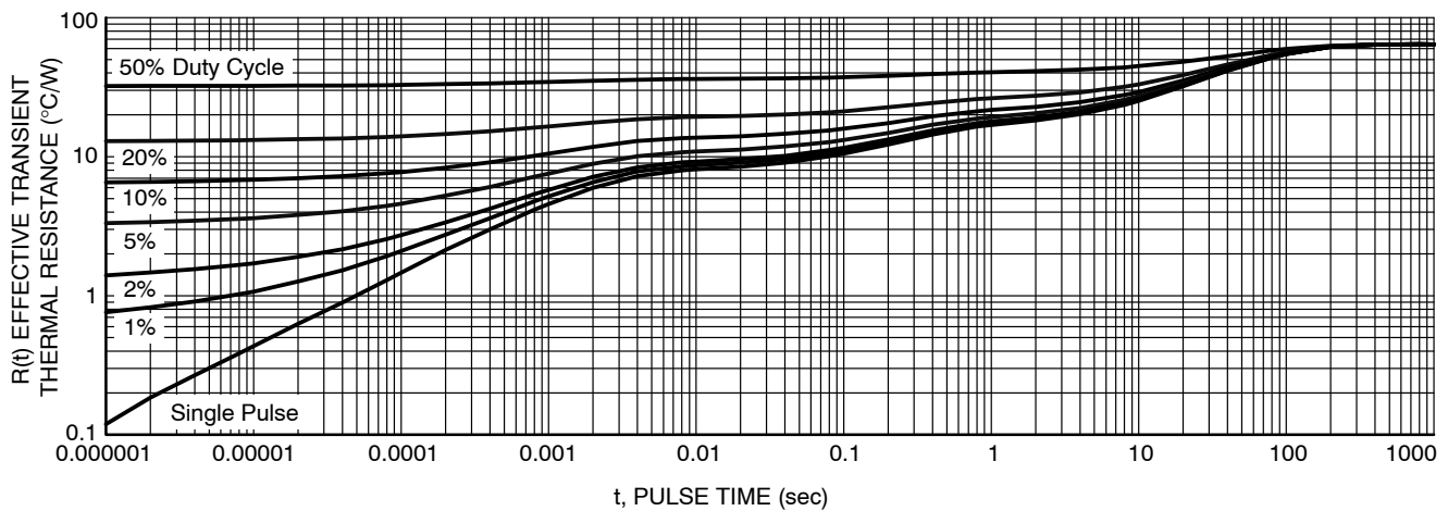
Figure 3. Thermal Resistance (FR-4 @ 645 mm², 1 oz. Cu trace)
