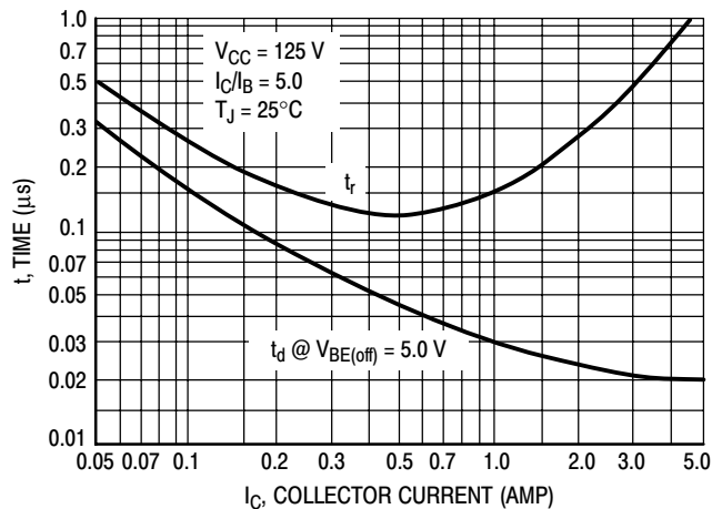
Figure 2. Turn-On Time
