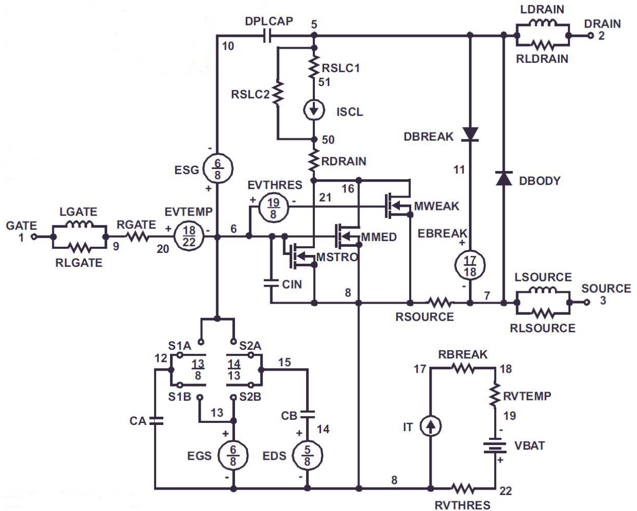
Figure 23. SABER Electrical Model
