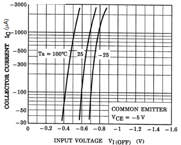
Fig. 9.4 RN2911EF I C -V I(OFF)
