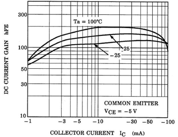
Fig. 10.8 RN2908 h_{FE}-I_C
