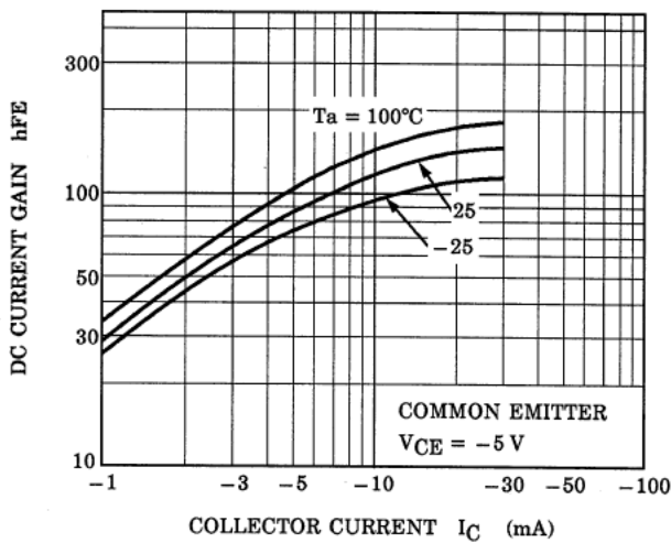
Fig. 10.9 RN2909 h_{FE}-I_C
