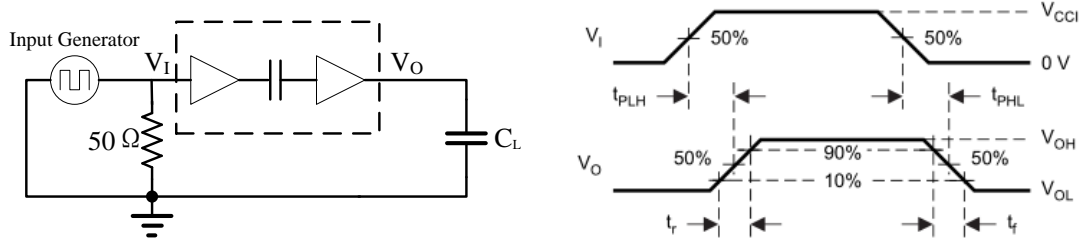
Figure 5.9 Switching Characteristics Test Circuit and Waveform
