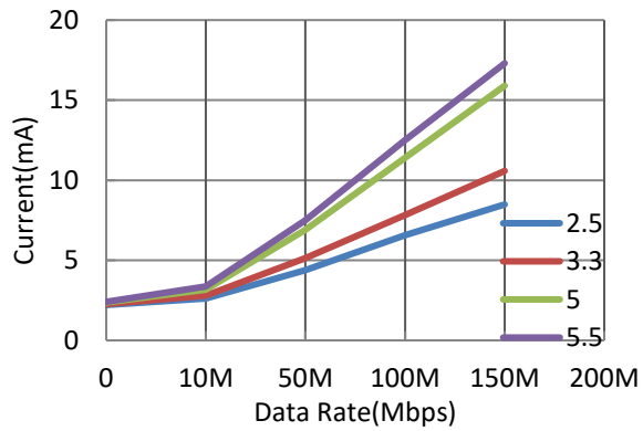
Figure 5.3 NSi8131 VDD1 Supply Current vs Data Rate
