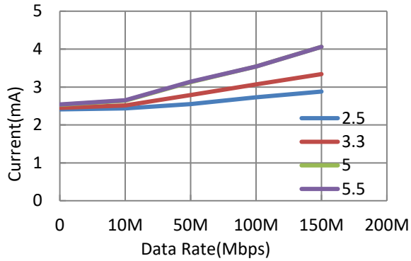
Figure 5.1 NSi8130 VDD1 Supply Current vs Data Rate
