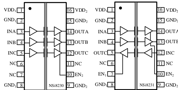
Figure 1.1 NSi8230W Package
