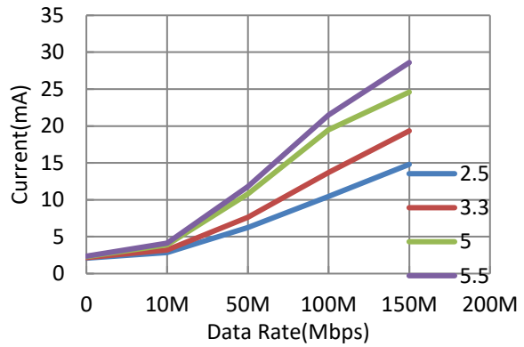
Figure 5.4 NSi8131 VDD2 Supply Current vs Data Rate
