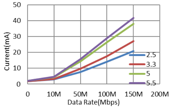
Figure 5.2 NSi8130 VDD2 Supply Current vs Data Rate
