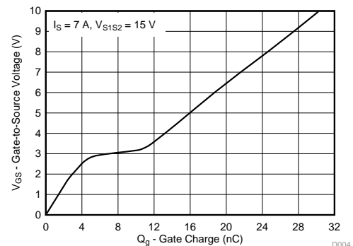
Gate Charge
