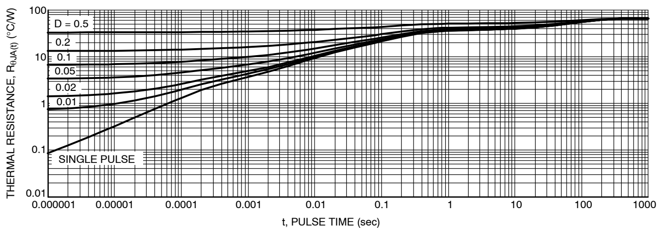
Figure 26. Thermal Response
