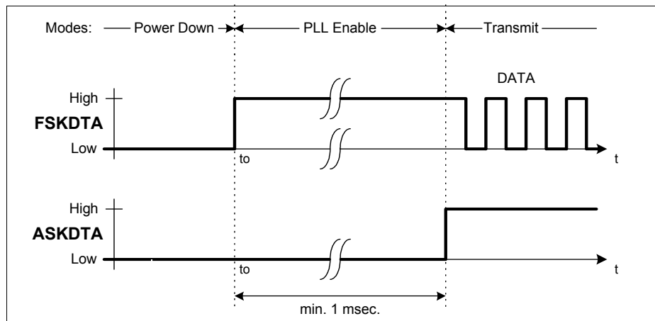
Figure 5 FSK Modulation
