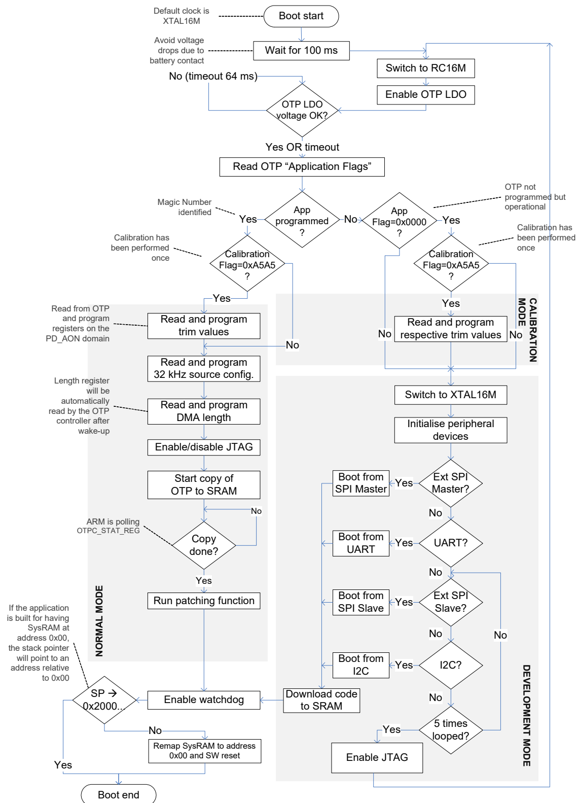
Figure 5: BootROM Sequence
