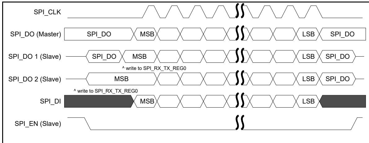
Figure 2: SPI Master/Slave, Mode 0: SPI_POL=0 and SPI_PHA=0
