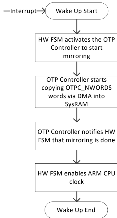
Figure 4: Wake-Up OTP Mirroring
