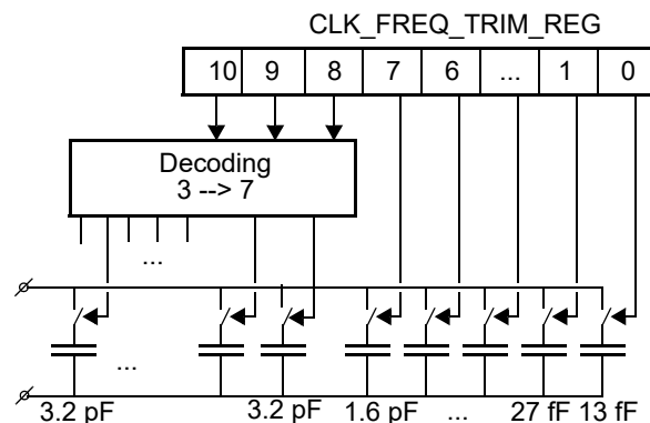
Figure 2: Frequency Trimming
