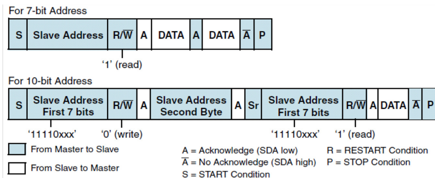
Figure 8: Master-Receiver Protocol
