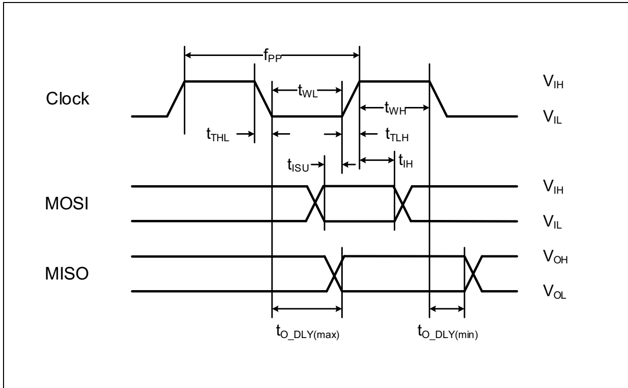
FIGURE 2-2: SPI PERIPHERAL INTERFACE TIMING
