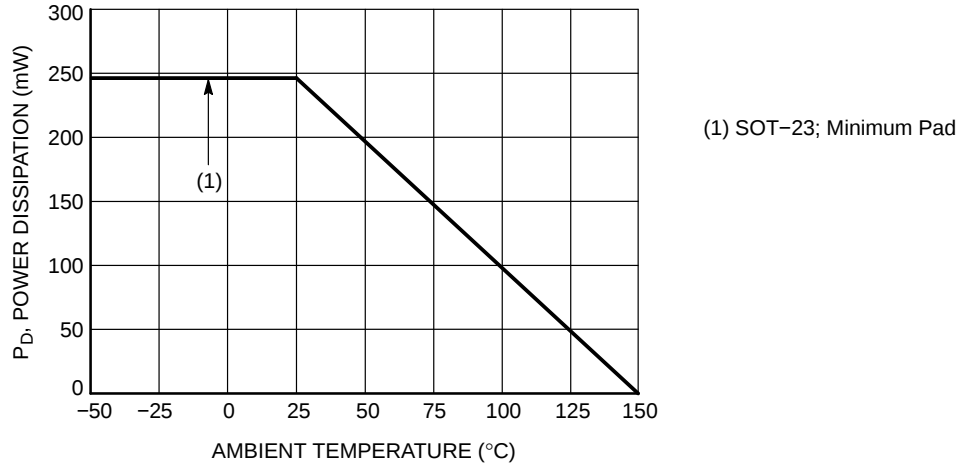
Figure 1. Derating Curve
