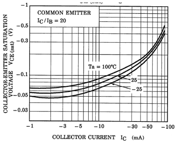
Fig. 10.23 RN2905 V_{CE(sat)}-I_C
