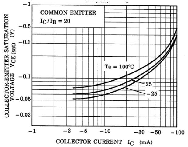
Fig. 10.20 RN2902 V_{CE(sat)}-I_C
