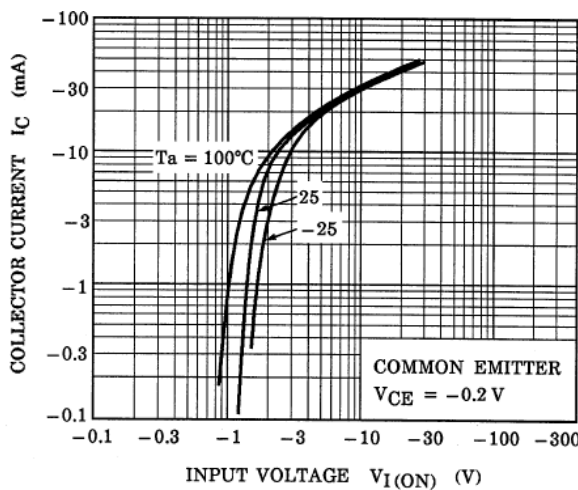
Fig. 10.3 RN2903 I_C - V_{I(ON)}
