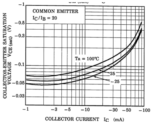
Fig. 10.24 RN1206 V_{CE(sat)}-I_C
