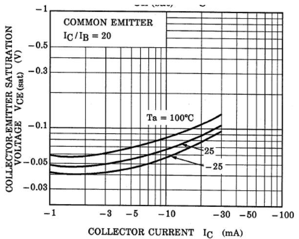
Fig. 10.22 RN2904 V_{CE(sat)}-I_C
