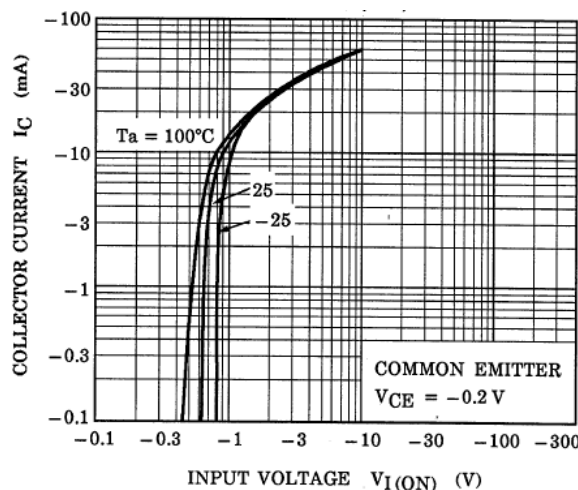
Fig. 10.5 RN2905 I_C - V_{I(ON)}
