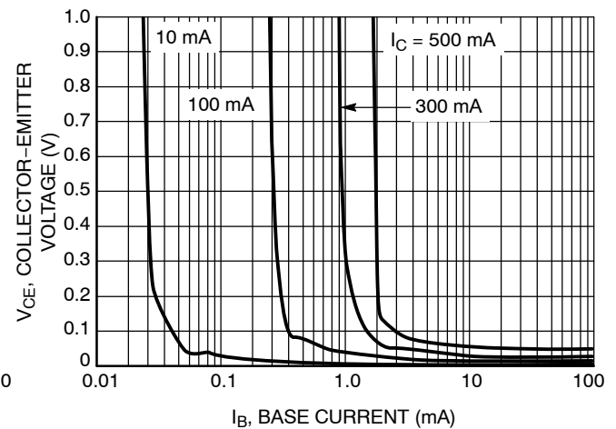
Figure 20. Saturation Region
