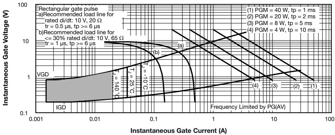
Fig. 8 - Gate Characteristics
