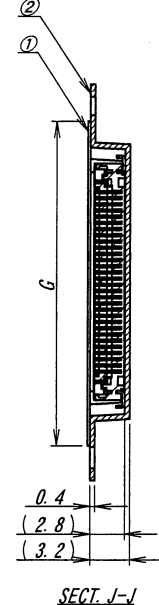
SECT. J-J
