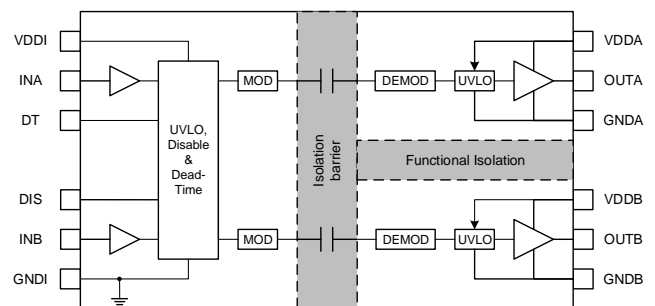
Figure 1. NSI6602 Block Diagram
