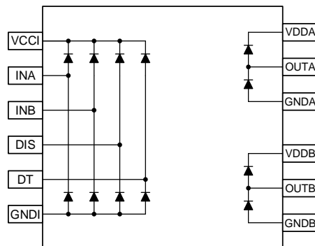
Figure 7.3 ESD Structure
