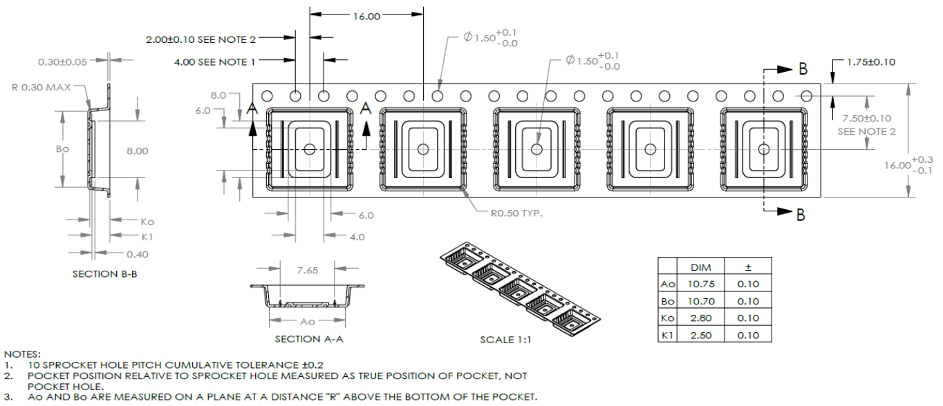
Figure 12.3 SOW16/SOW14 Reel Information
