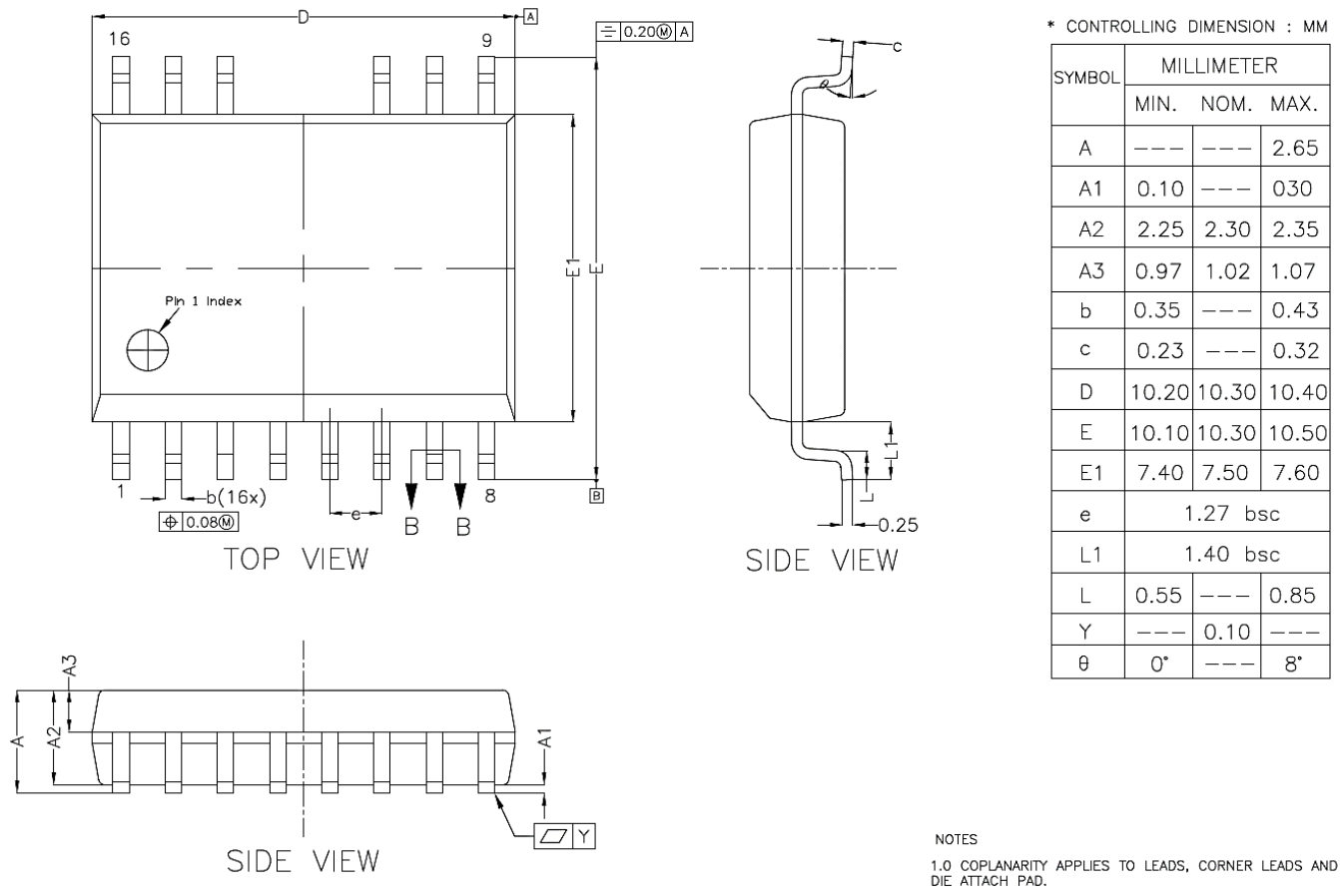
Figure 9.3 SOW14 Package Shape and Dimension
