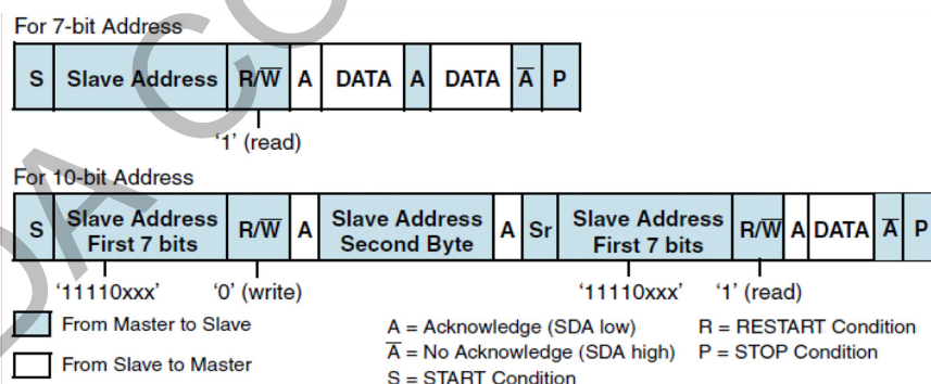
Figure 25: Master-Receiver Protocol
