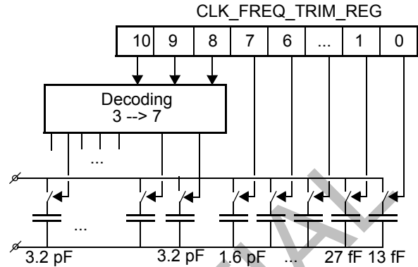
Figure 15: Frequency Trimming
