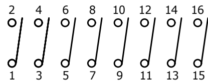
▲ CIRCUIT - 8 POSITION
