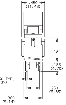
SNAP-IN
