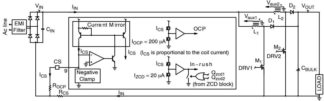
Figure 9. Current Sense Block
