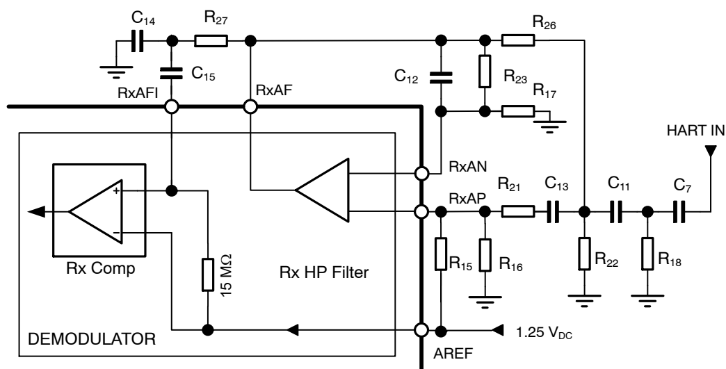
Figure 14. Receive Filter
