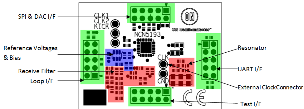
Figure 3. Board Drawing with Indication of Different Sections
