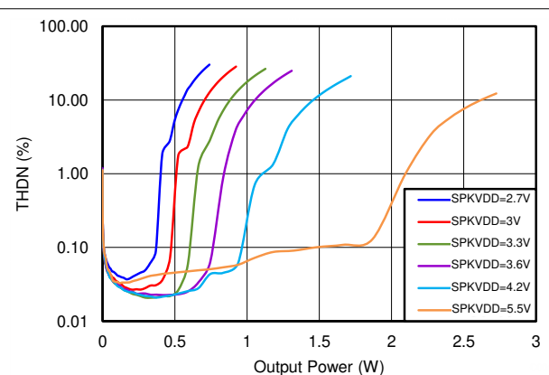
Figure 8-3. Total Harmonic Distortion + Noise vs 4-Ω Speaker Power
