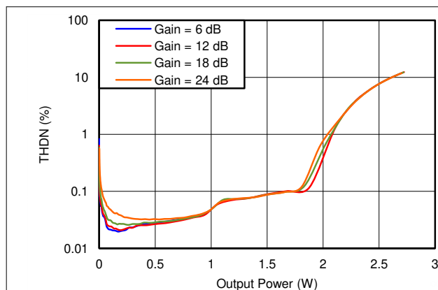
Figure 8-2. Total Harmonic Distortion + Noise vs 4-Ω Speaker Power
