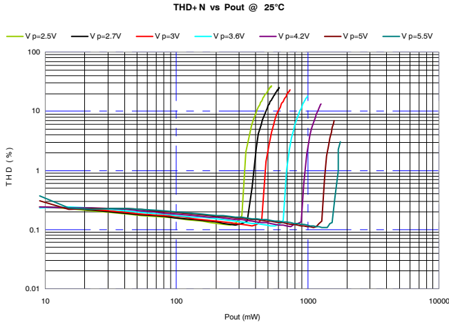
Figure 4. THD vs. P_{OUT} , R_L = 8 \Omega , f = 1 \text{ kHz}
