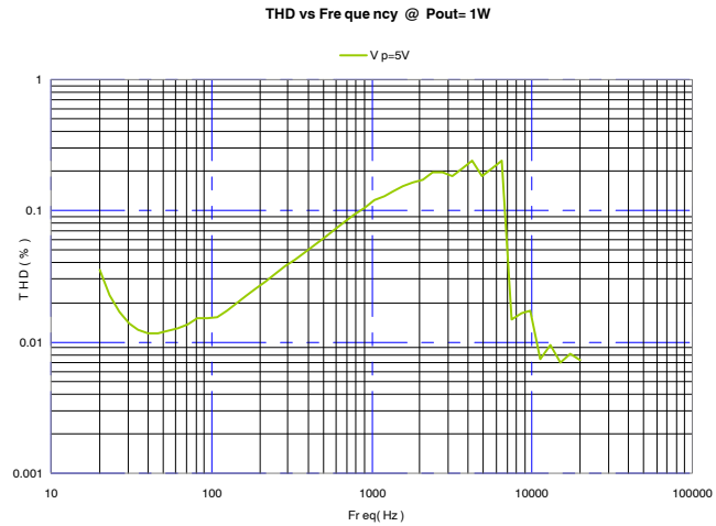
Figure 8. THD vs. Frequency, R_L = 8 \Omega , P_{OUT} = 1 \text{ W}
