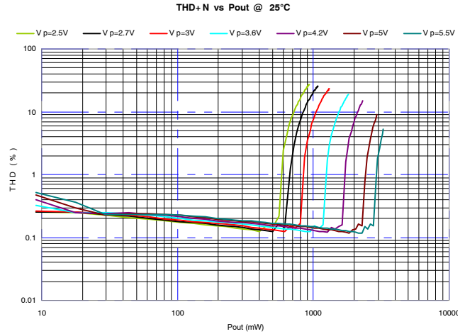
Figure 5. THD vs. P_{OUT} , R_L = 4 \Omega , f = 1 \text{ kHz}
