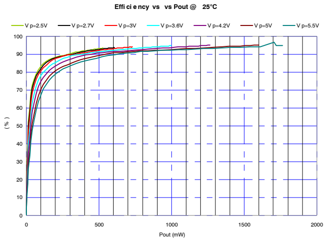
Figure 6. Efficiency vs. P_{OUT} , R_L = 8 \Omega , f = 1 \text{ kHz}
