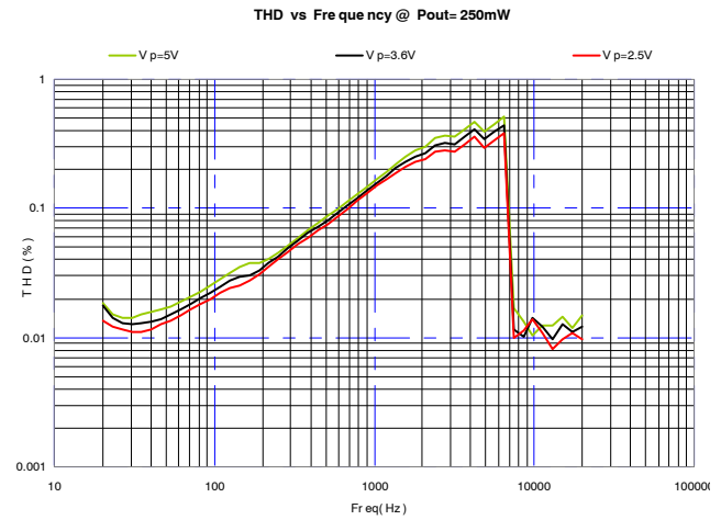
Figure 7. THD vs. Frequency, R_L = 8 \Omega , P_{OUT} = 250 \text{ mW}
