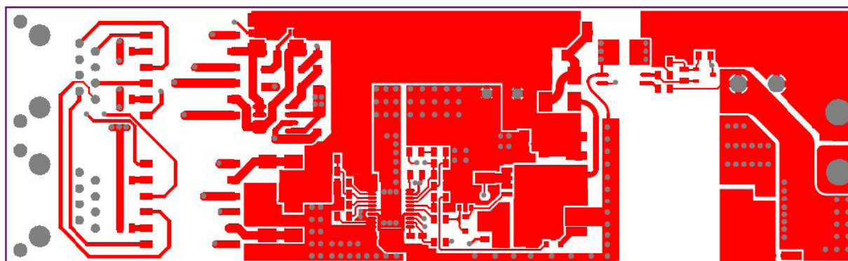
Figure 3. Layout (Top)
