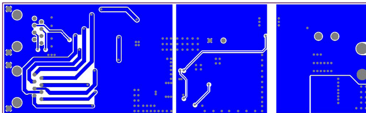
Figure 4. Layout (Bottom)
