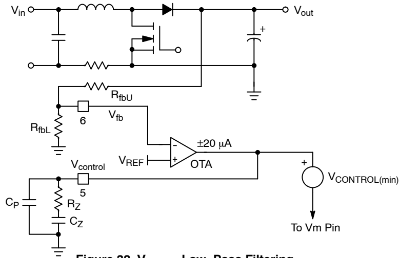
Figure 38. V_{\text{control}} Low-Pass Filtering
