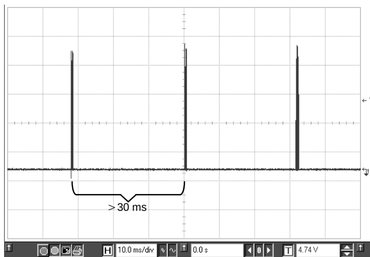
Figure 21. The burst frequency becomes so low that it is difficult to keep an adequate level on the auxiliary V_{CC} \dots
