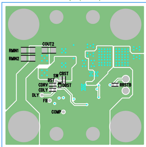
Figure 15. Bottom View
