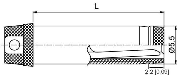
RECOMMENDED PLUG
