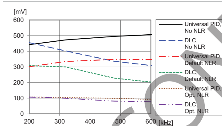
Load transient vs. Switch Frequency
