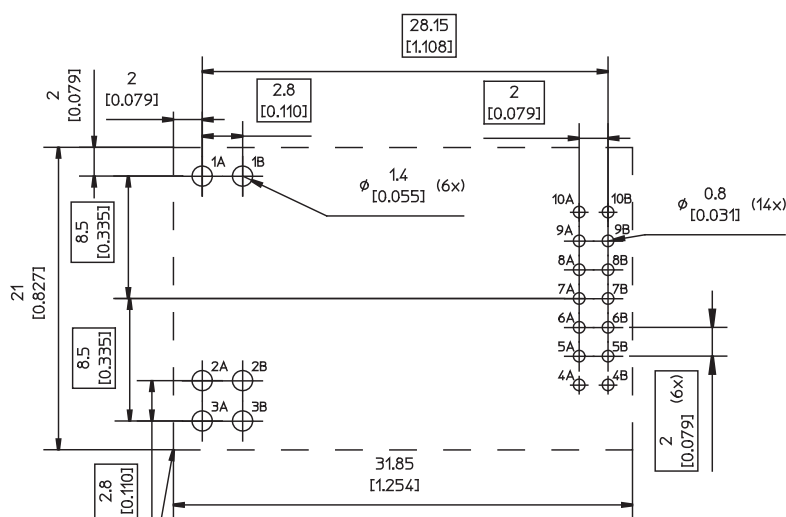
TOP VIEW Pin positions according to recommended footprint
