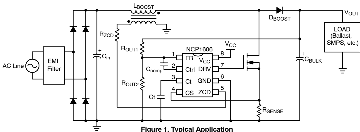
Figure 1. Typical Application
