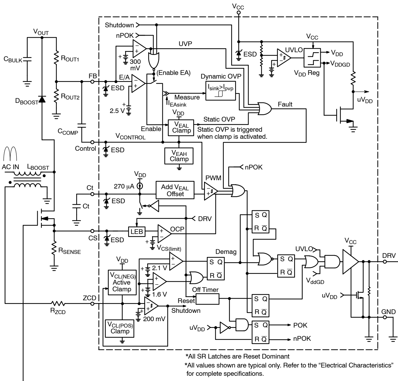
Figure 2. Block Diagram
