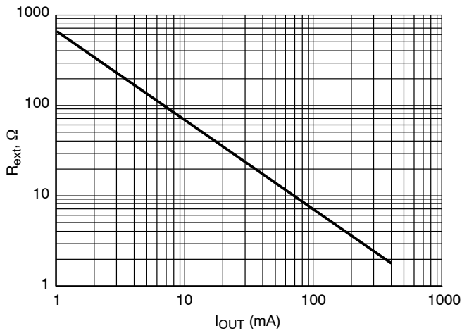
Figure 1. Output Current ( I_{\text{OUT}} ) vs. External Resistor ( R_{\text{ext}} )
