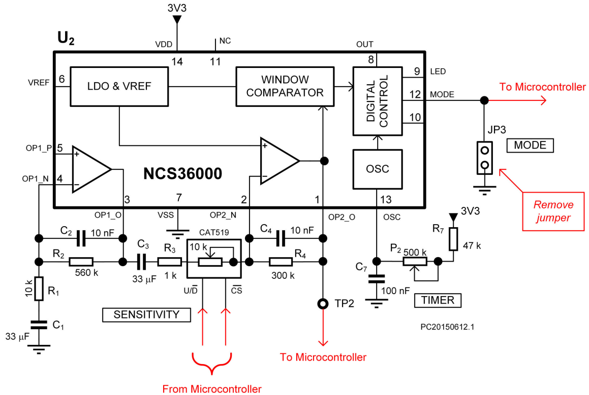
Figure 7. Schematic Diagram
