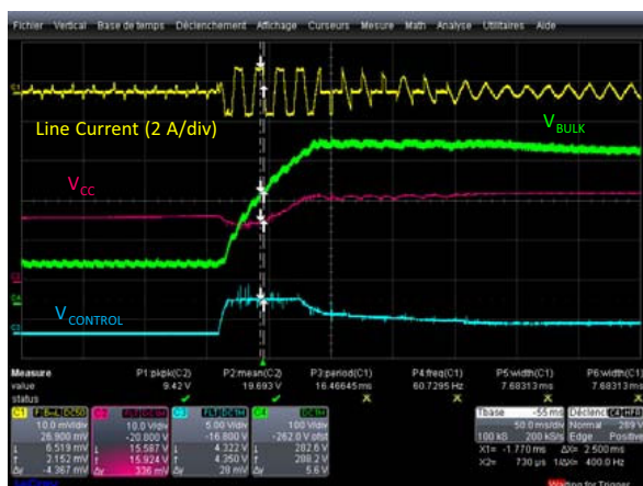
a) Start of operation when V_{in,rms} exceeds (V_{in,rms})_{BOH} (NCP1612B)
