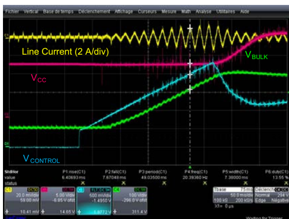
b) Start of operation when V_{in,rms} exceeds (V_{in,rms})_{BOH} (NCP1612A)
