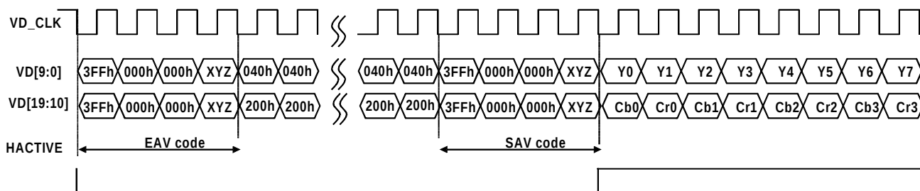
FIGURE 7. BT.1120 FORMAT
