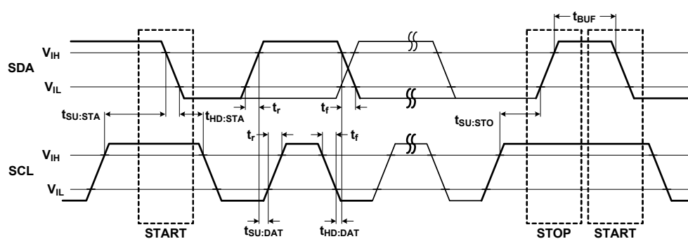
FIGURE 19. I 2 C TIMING DEFINITIONS
