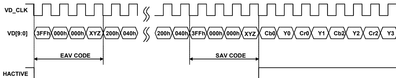
FIGURE 4. BT.656 FORMAT
